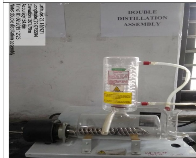
1 Double Distillation Assembly
